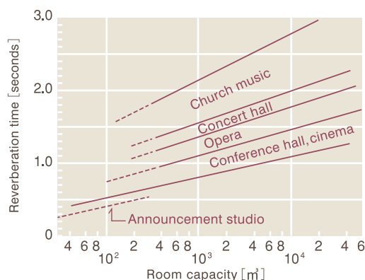
Fig.9. Scope of optimal reverberation time (500 Hz)
