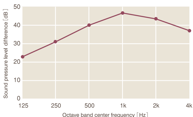
Fig.5. Sound insulation (between exterior and the cloisters)
