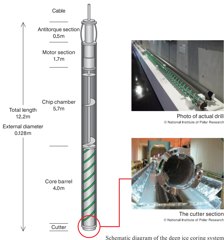
Schematic diagram of the deep ice coring system
