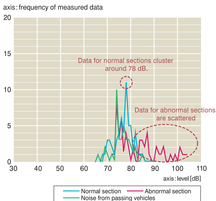
Fig.5. Frequency distribution at 2.5 KHz band
