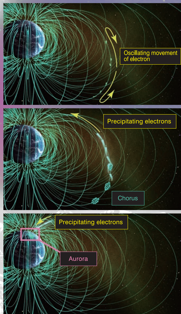
Fig.1. Mechanism generating pulsating auroras © ERG science team
